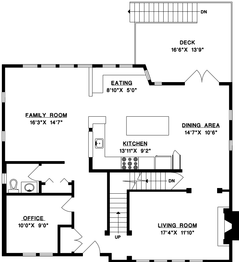
MAIN FLOOR
