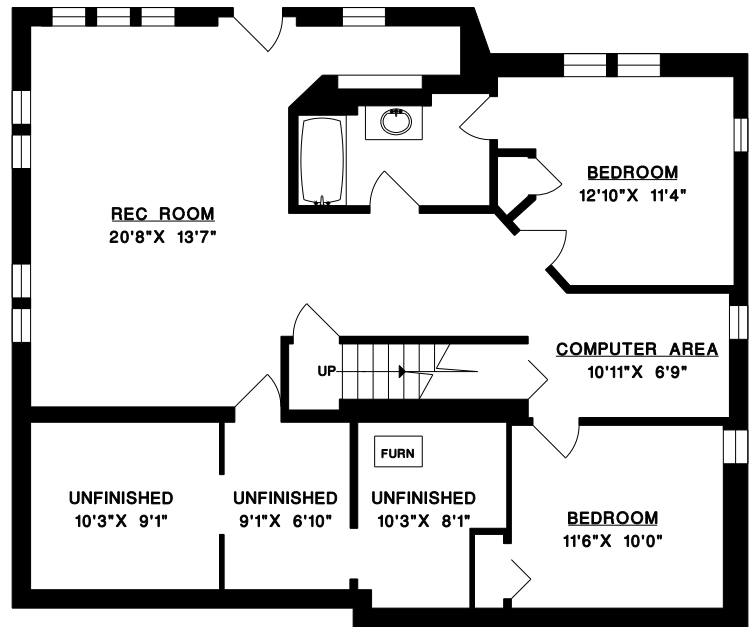
LOWER FLOOR
