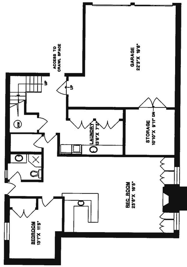
LOWER FLOOR
